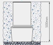
Retrofit - Glasdon Ground Socket ("Round" Socket)
