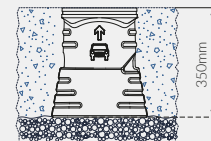
Retrofit - Glasdon LockFast™ Socket ("Square" Socket)
