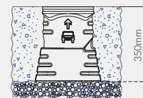
Retrofit - Glasdon LockFast™ Socket ("Square" Socket)
